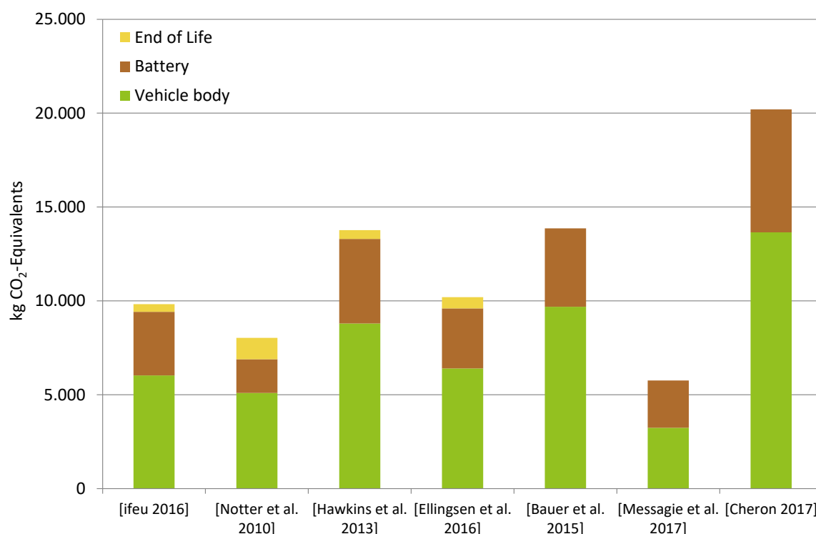
Figure A25: GHG emission results for the production of electric vehicles from selected LCA studies
