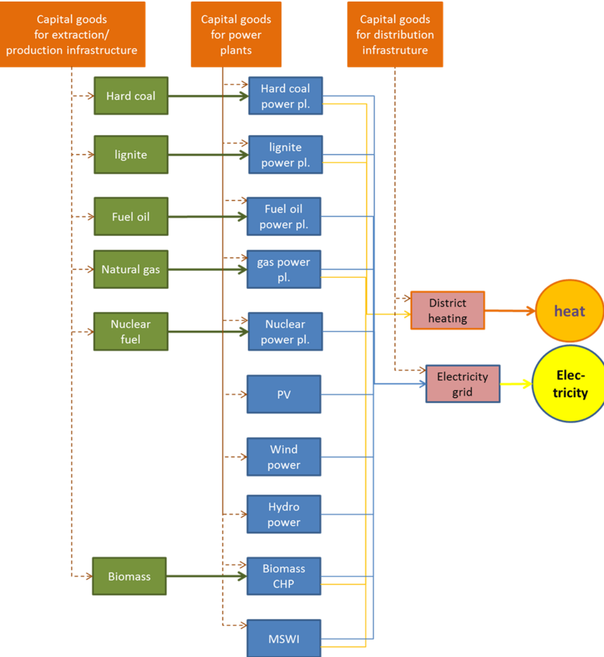
Figure A54: Schematic structure of the Umberto electricity model, subdivided into the modules fuel pre-chains (green), power plants (blue), distribution (lilac), capital goods (brown)
