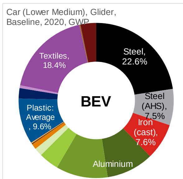
Figure 5.61: Breakdown of (i) mass (kg) and (ii) GWP impacts, for Lower Medium Car materials in the Glider (common to all powertrains types), Baseline scenario
